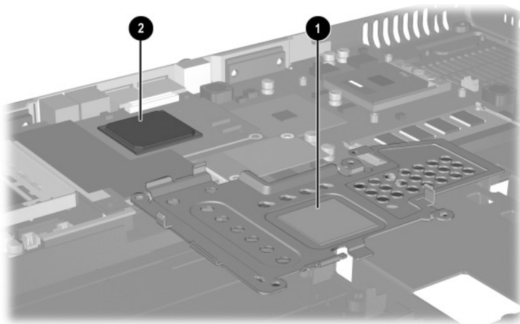
Replacing the Thermal Pads on the VGA Board and Shield
